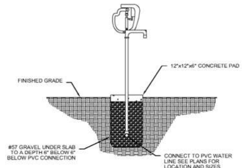
FREEZE PROOF YARD HYDRANT
