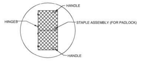
WET WELL HATCH DETAIL NOT TO SCALE
