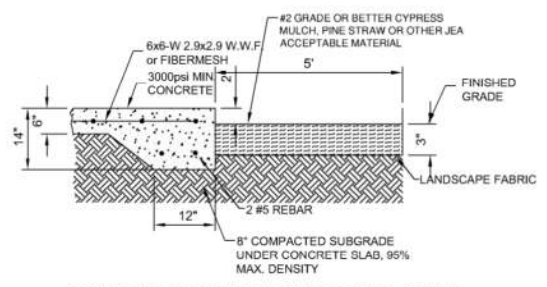
CONCRETE SLAB AND GROUND COVER DETAIL NOT TO SCALE
