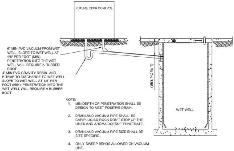
ODOR CONTROL DRAIN AND VACUUM CONNECTION TO WET WELL DETAIL NOT TO SCALE
